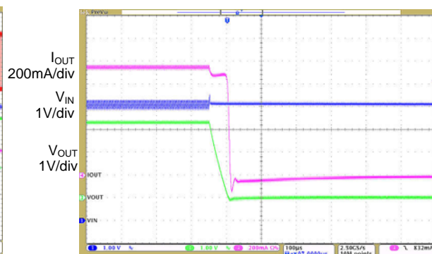
Time 100μs/div
