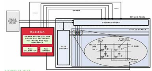
FIGURE 1. TYPICAL APPLICATION: TFT-LCD REFERENCE VOLTAGE GENERATOR
