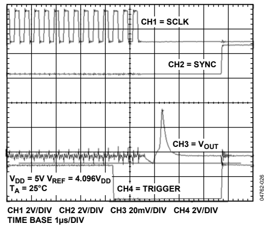
Figure 26. Exiting Software Power-Down Glitch
