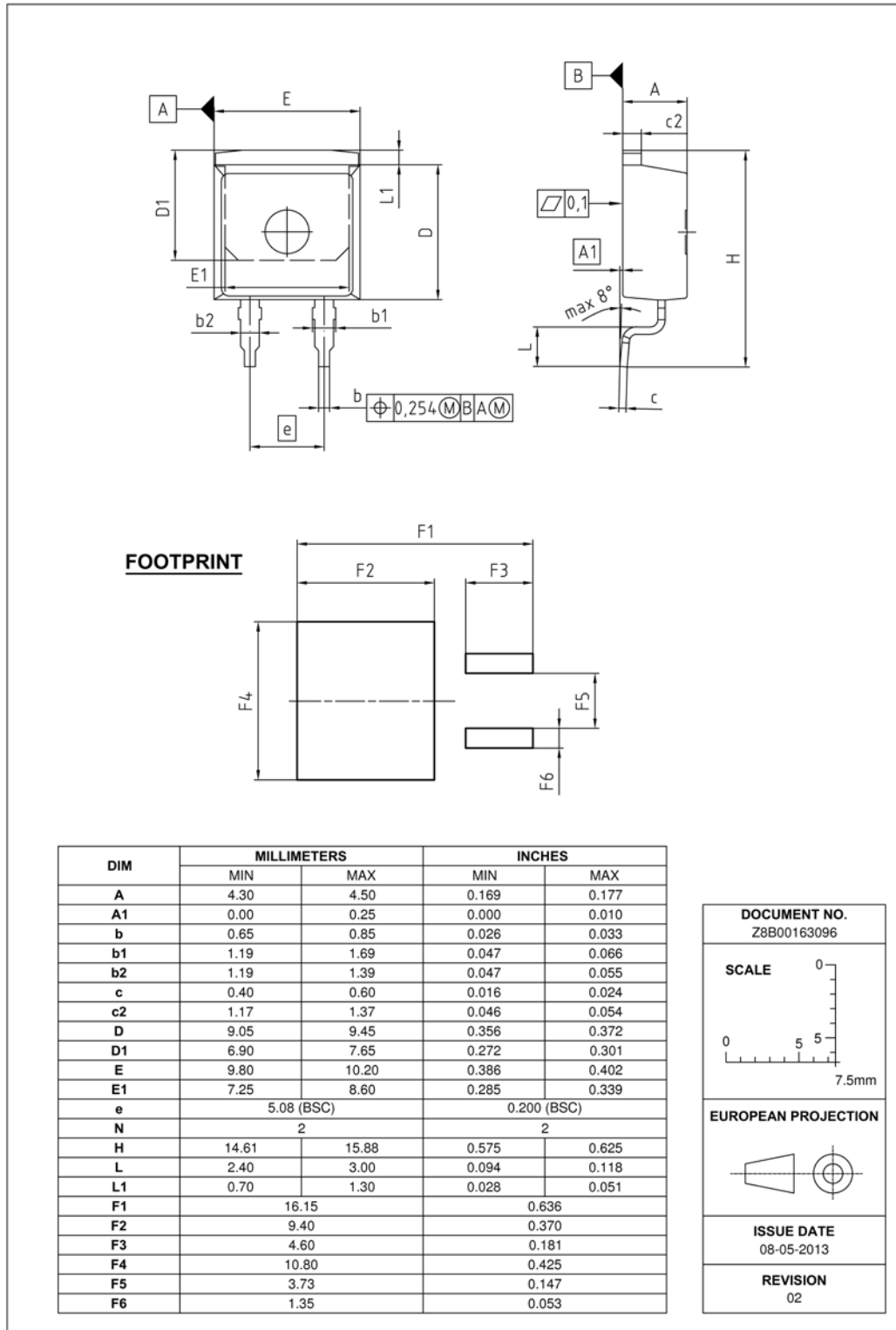
Figure 1 Outlines TO-220, dimensions in mm/inches
