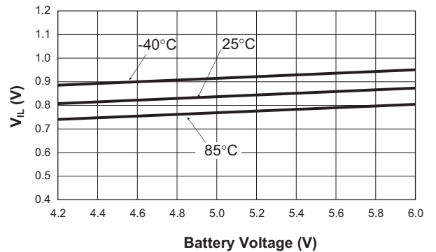
V_{IL} vs. Supply Voltage (ENBAT = Falling)
