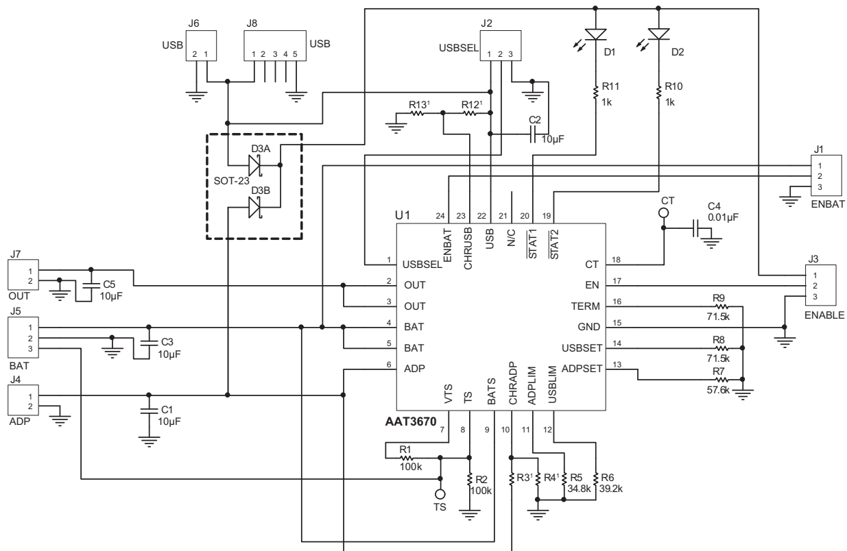
Figure 8: AAT3670 Evaluation Board Schematic.
