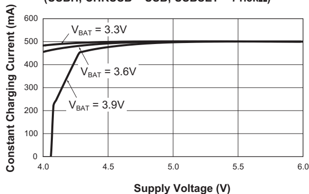
Constant Charging Current vs. Supply Voltage (USBH; CHRUSB = USB; USBSET = 71.5kΩ)
