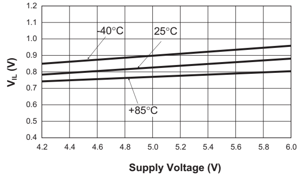
V_{IL} vs. Supply Voltage (ADP or USBL or USBH; EN = Falling)
