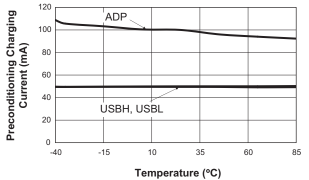
Preconditioning Charging Current vs. Temperature ( V_{IN} = 5.0V )
