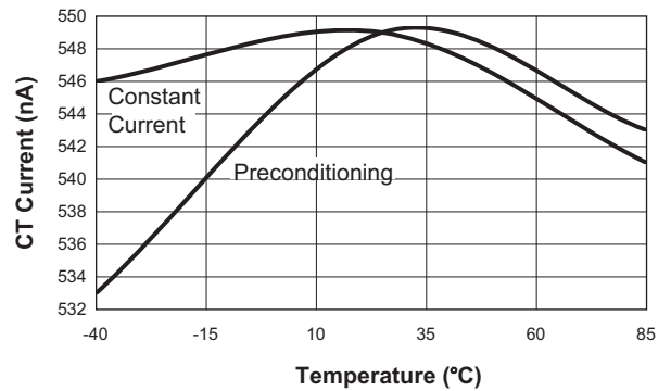
CT Current vs. Temperature ( C_T = 0.1\mu F )
