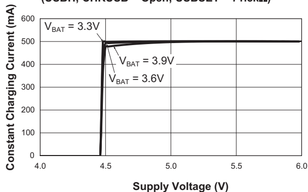
Constant Charging Current vs. Supply Voltage (USBH; CHRUSB = Open; USBSET = 71.5kΩ)
