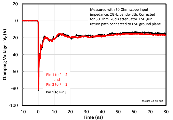
ESD Clamping (-8kV Contact per IEC 61000-4-2)
