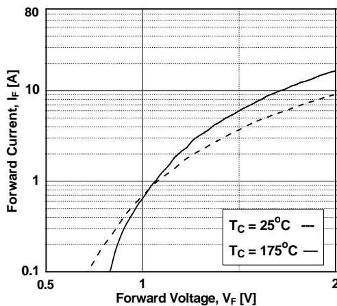
Figure 18. Forward Characteristics
