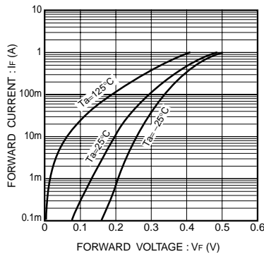
Fig.8 Forward characteristics
