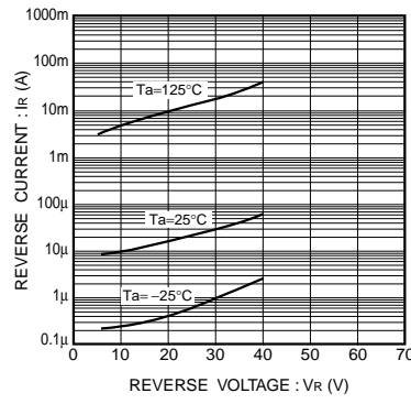
Fig.9 Reverse characteristics
