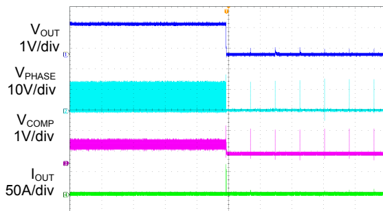
Time 10ms/div
