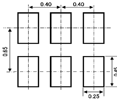
Fig. 7.1 Land Pattern Dimensions (Unit: mm)
